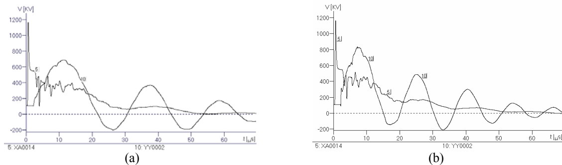
Fig. 7. a) Voltage waveform in input of substation due to lightning arising on Tower 3, a) with tower resistance of 20\ \Omega - when substation has not arrester and CVT), b) with tower resistance of 20\ \Omega - when substation has CVT and has not arrester)
